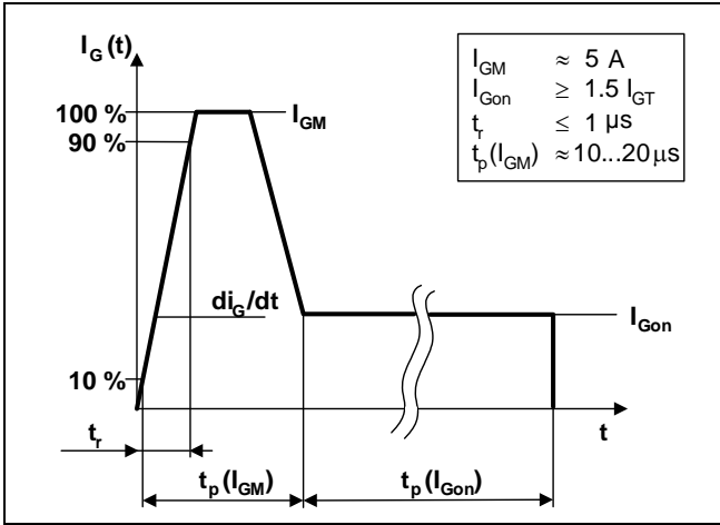
Fig. 6 Recommended gate current waveform
