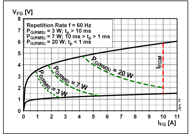
Fig. 7 Max. peak gate power loss
