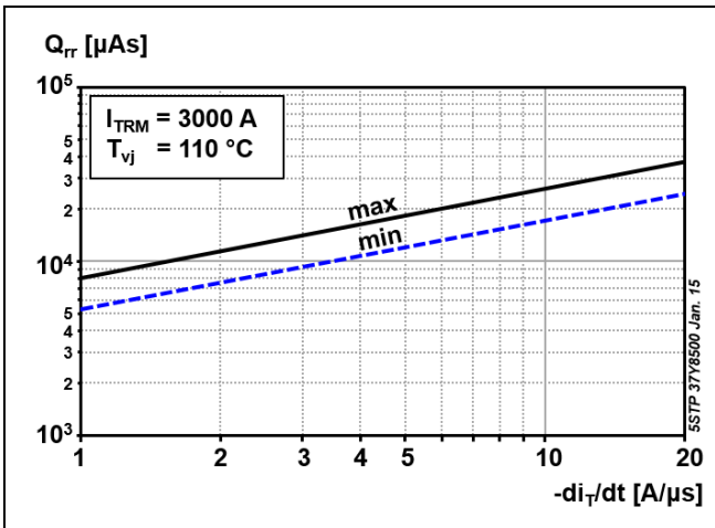
Fig. 8 Reverse recovery charge vs. decay rate of on-state current
