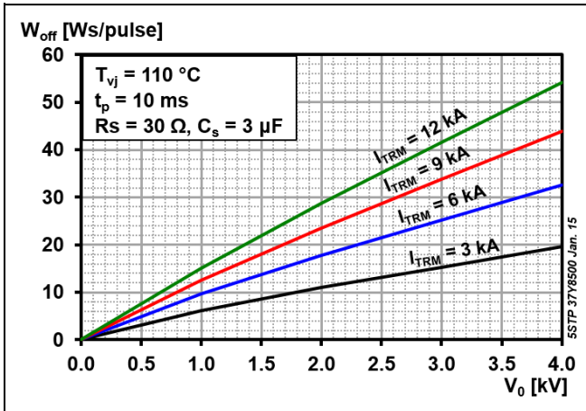
Fig. 10 Turn-off energy, half sinusoidal waves
