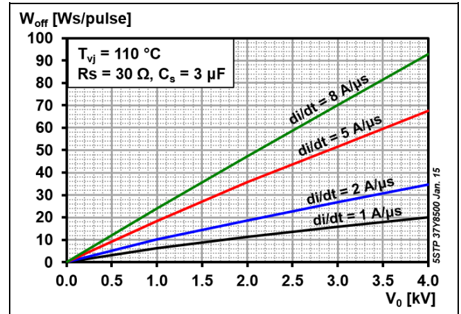
Fig. 11 Turn-off energy, rectangular waves
